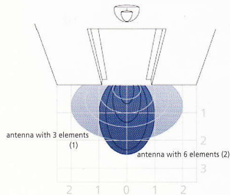
Sensing fields in accordance with type of antenna and sensitivity mounting height : 2.2m
