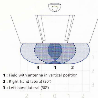
Sensing fields in accordance with lateral position of antenna mounting height : 2.2m
